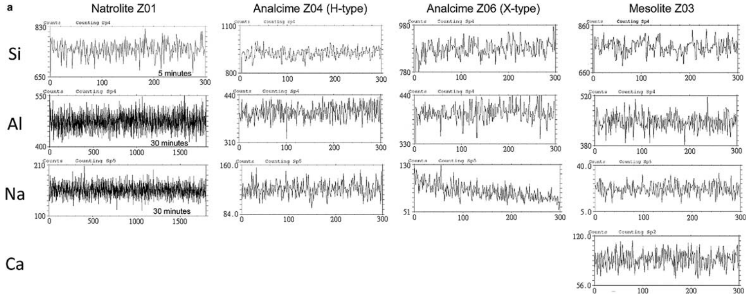
FIG. 4. ( a above and b next page). Test 4: Selected count rate profiles per element per reference zeolite, collected over 300 s (and 1800 s for natrolite, Z01) using a 2 nA, defocused 20 \mu m beam. The count-sampling interval was every 200 ms. All other reference samples displayed steady, horizontal profiles for every major element in their respective mineral formulae. For clarity only the upper and lower x-axis figures are given.
